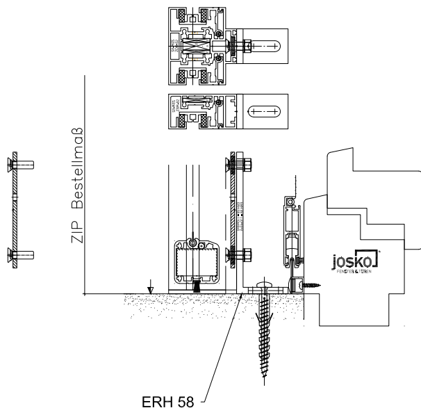
Kasten 105 RR
