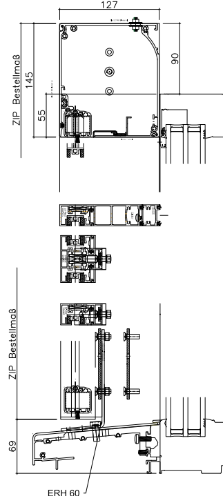
Kasten 127 RR
