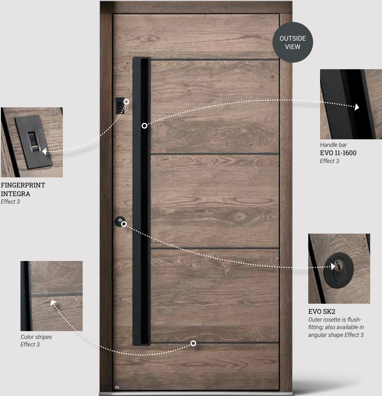
DE.NIRO 4 Nevos Natur – SET outside Surface knotty oak N06 silver grey brushed Stripes Color Effect 3 Handle bar EVO 11-1600 Effect 3 Motor lock Genius CA with Integra 1 BT/App
